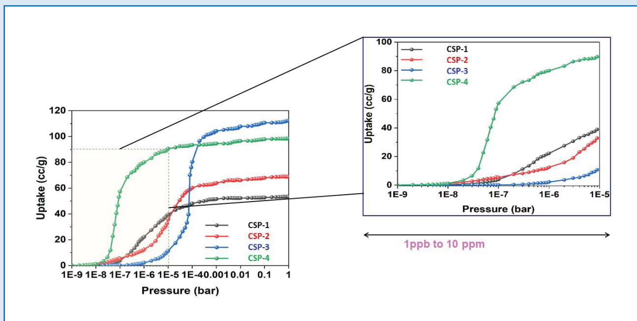
Figure 7: Single component adsorption isotherms at 298 K of NDMA nitrosamine in 4 nanoporous materials engineered at Aptar Active Material Science
