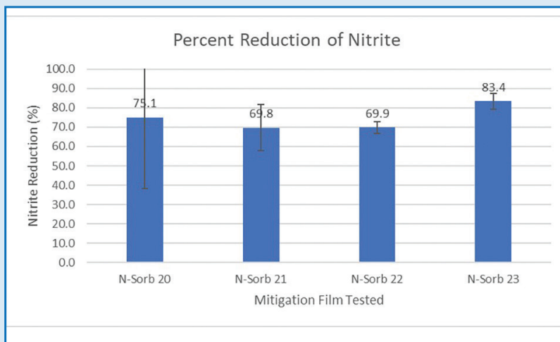
Figure 7: Percent reduction of nitrite in MCC tablets sealed with N-Sorb SM mitigation films when compared to control sample
