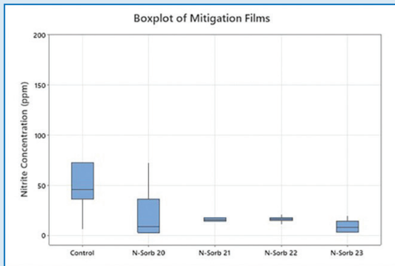
Figure 6: Nitrite Concentration (ppm) vs. N-Sorb SM mitigation films in the sample headspace of vials sealed with MCC tablets
